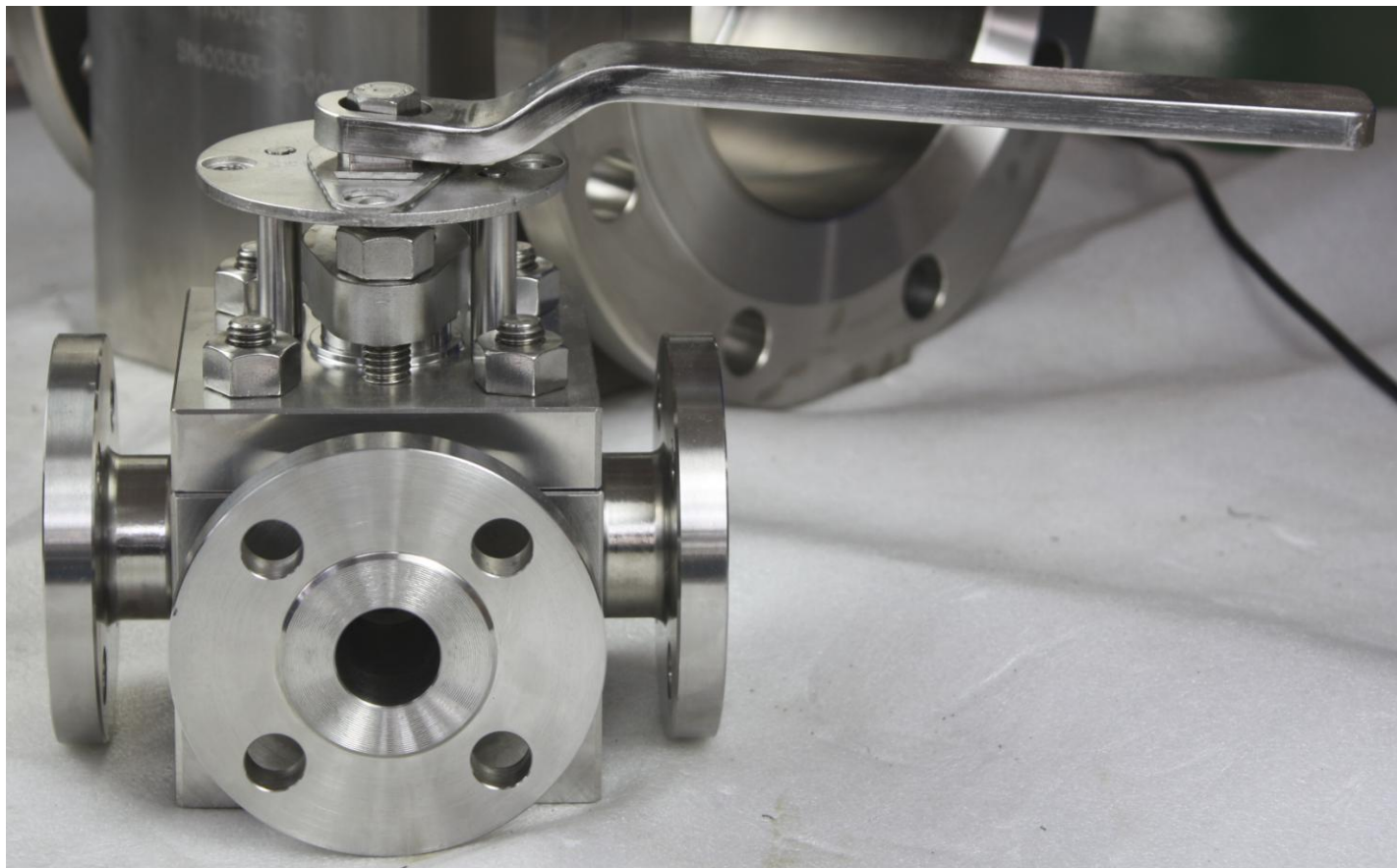
b) Zirconium 3-Way Plug Valve
