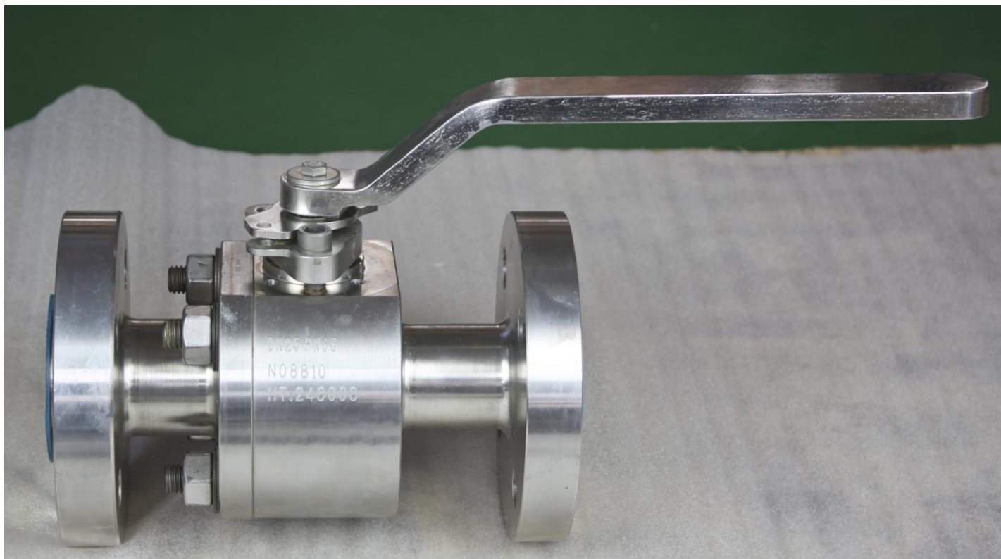
h) High Temp, Metal Seated Floating Ball Valve
