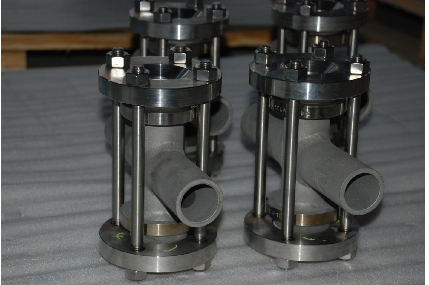
d) Hastelloy Sight Glass
